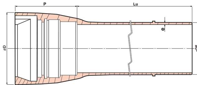
Q.R Flex DN 150-600 mm in K Class-EN 545:2007
